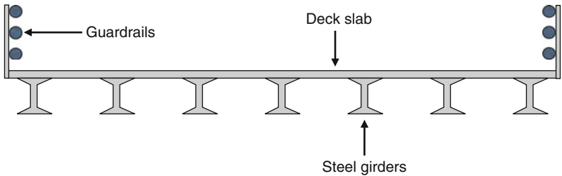
Fig. 6.2 The highway bridge – cross section
