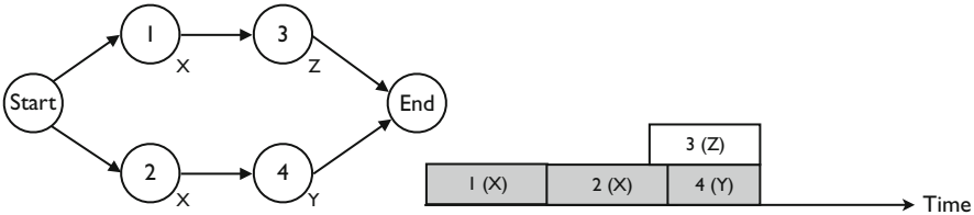
Fig. 10.9 An unbuffered resource feasible schedule (CC = 1-2-4)
